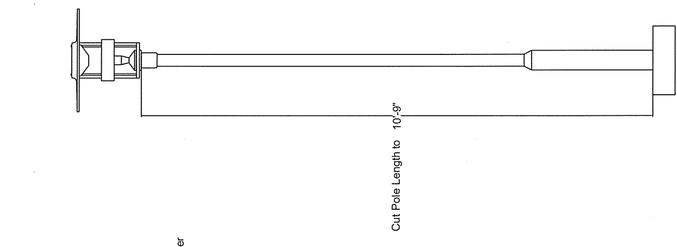
New Albertslund Fixture on New 12' 5-3 Stepped Pole Cut to Match Height of Existing Lights
